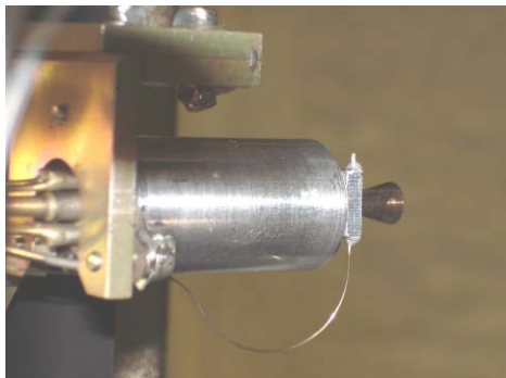
Fig. 11: FBG Sensors integrated with SSTL Propulsion Subsystem.
