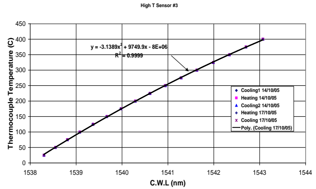
Fig. 7: High-T sensor calibration after repeated thermal cycling.
