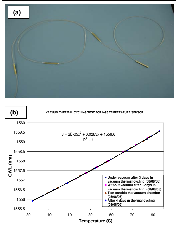
Fig. 9: (a) photograph of a packaged flight FBG T-sensor line with protective cabling and four sensors, (b) test results for one of the FSD FBG T-sensors.
