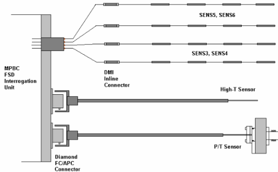
Fig. 4: Schematic of FSD fiber-optic sensor signal harness.
