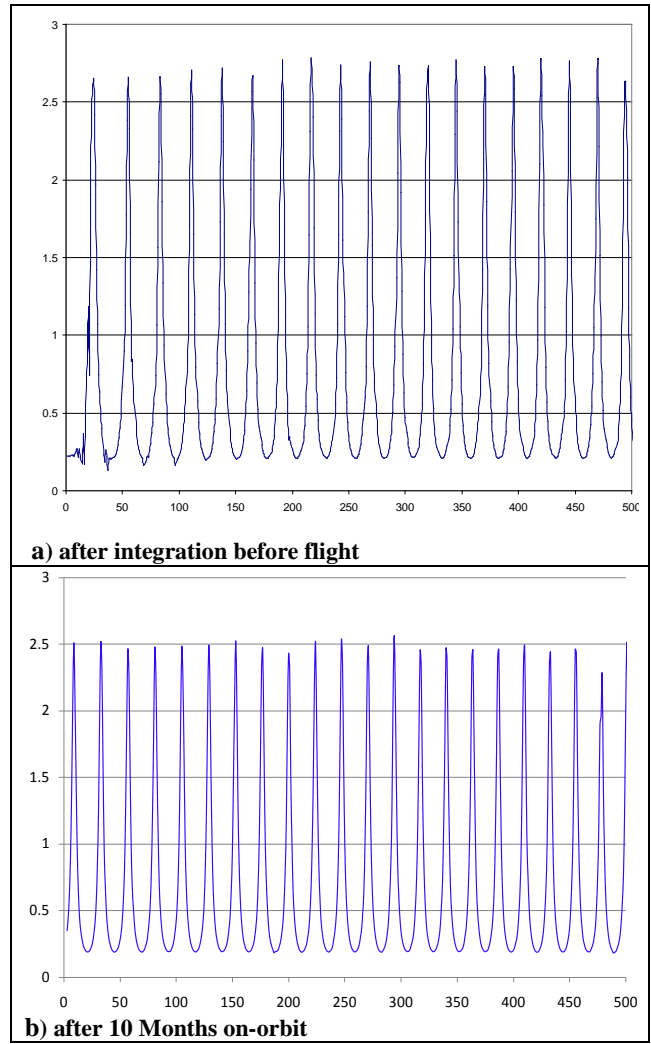
Fig. 13 : Fixed Fabry-Perot signal a) before the flight and b) after 10 Months on orbit.
