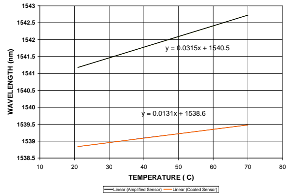
Fig. 8: Measured temperature response of bare FBG (red curve) and packaged FBG with MEMS-amplified thermal sensitivity (dark curve).
