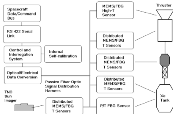
Fig. 1: Block diagram of the Fiber-optic Sensor Demonstrator for Proba 2.
