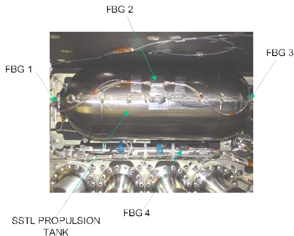
Fig.10: FBG Sensors integrated with SSTL Propulsion Subsystem.
