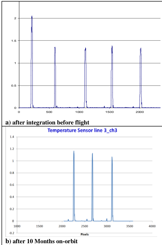
Fig.14: Readout scan of installed sensor line TS-003 a) on ground and b) after 10 months on-orbit.
