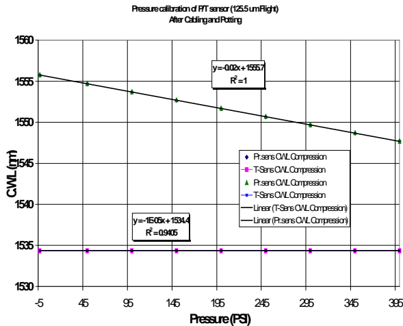
Fig. 6: Response of the P/T pressure-sensing and temperature sensing FBGs to the applied pressure.
