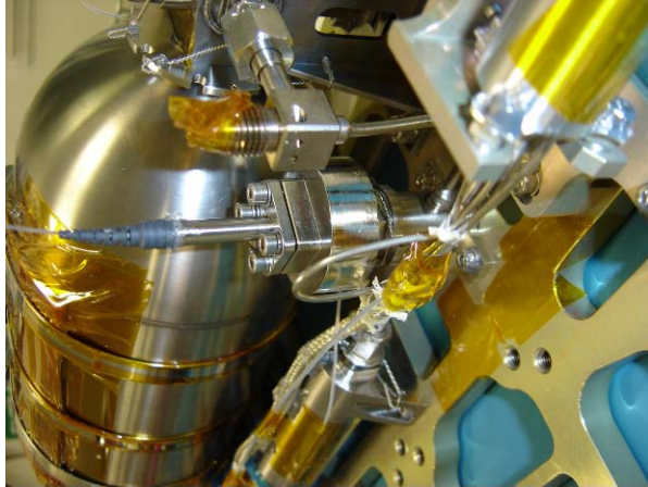
Fig. 5: Photograph of flight P/T sensor integrated with the SSTL propulsion system for Proba-2.
