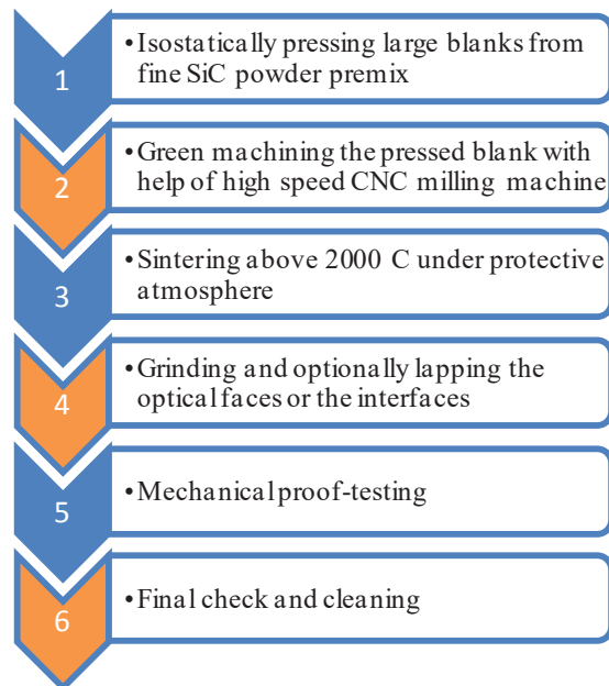
Fig. 3. Manufacturing process for monolithic sintered SiC parts
