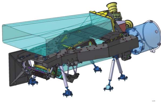
Fig. 4. Overview of the Sentinel-2 Multi Spectral Instrument (MSI)
