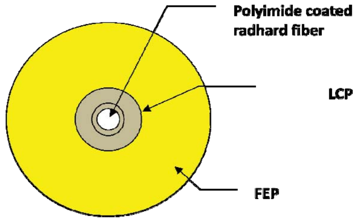
Figure 1. Design of RAVNOC
