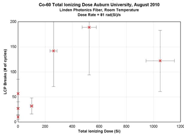
Figure 5. Flex Cycles till LCP Breakage vs. Dose
