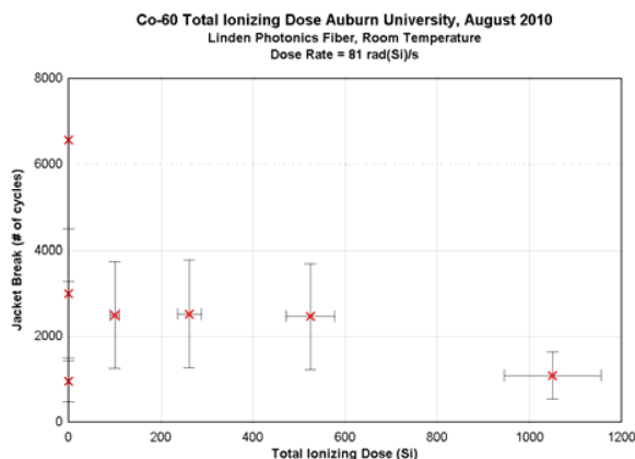
Figure 6. Flex Cycles till Outer Jacket Breakage vs. Dose
