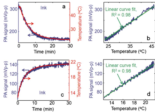
Fig. 3 (a) PA signal and actual temperature of diluted black ink solution ( \mu_a=30\text{ cm}^{-1} ) as the heated sample was allowed to come to room temperature, (b) PA signal versus temperature, which shows almost a linear relationship. Green line is the linear curve fitting with an R^2 of 0.98. (c) PA signal and the actual temperature of ink solution as cold solution was allowed to come to room temperature, (d) PA signal versus temperature, which shows almost a linear relationship. Green line is the linear curve fitting with an R^2 of 0.98. (Color online only.)
