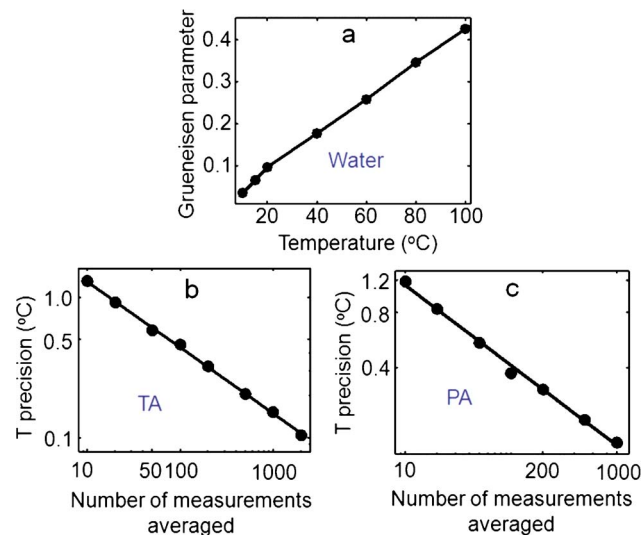
Fig. 4 (a) Variation of the Grueneisen parameter of water with temperature. 31,32 (b) Temperature precision versus number of measurements averaged for TA measurements in log-log scale. The plot shows a linear curve with a slope of -0.47 . (c) Temperature precision versus number of measurements averaged for PA measurements in log-log scale. The plot shows a linear curve with a slope of -0.44 .
