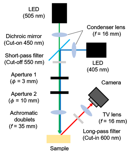
Fig. 1 Setup for the fluorescence observation. f is the focal length, and \phi is the aperture diameter. The excitation lights of dual wavelengths of 405 and 505 nm can be switched. Uniform light is irradiated to a sample surface with this optical system based on Kohler illumination. The long-pass filter is set in front of the TV lens to obtain only fluorescence of PpIX.
